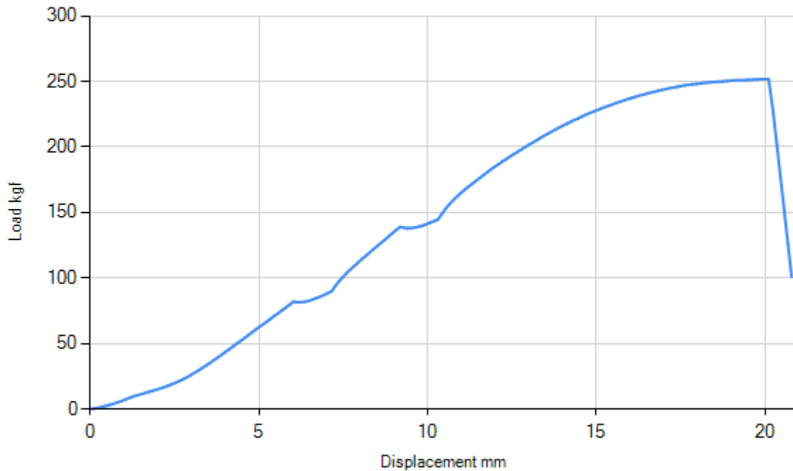
Load Vs Displacement
